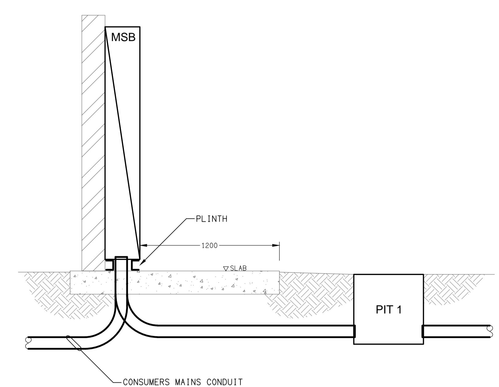
DETAIL A MSB SECTION VIEW NOT TO SCALE
