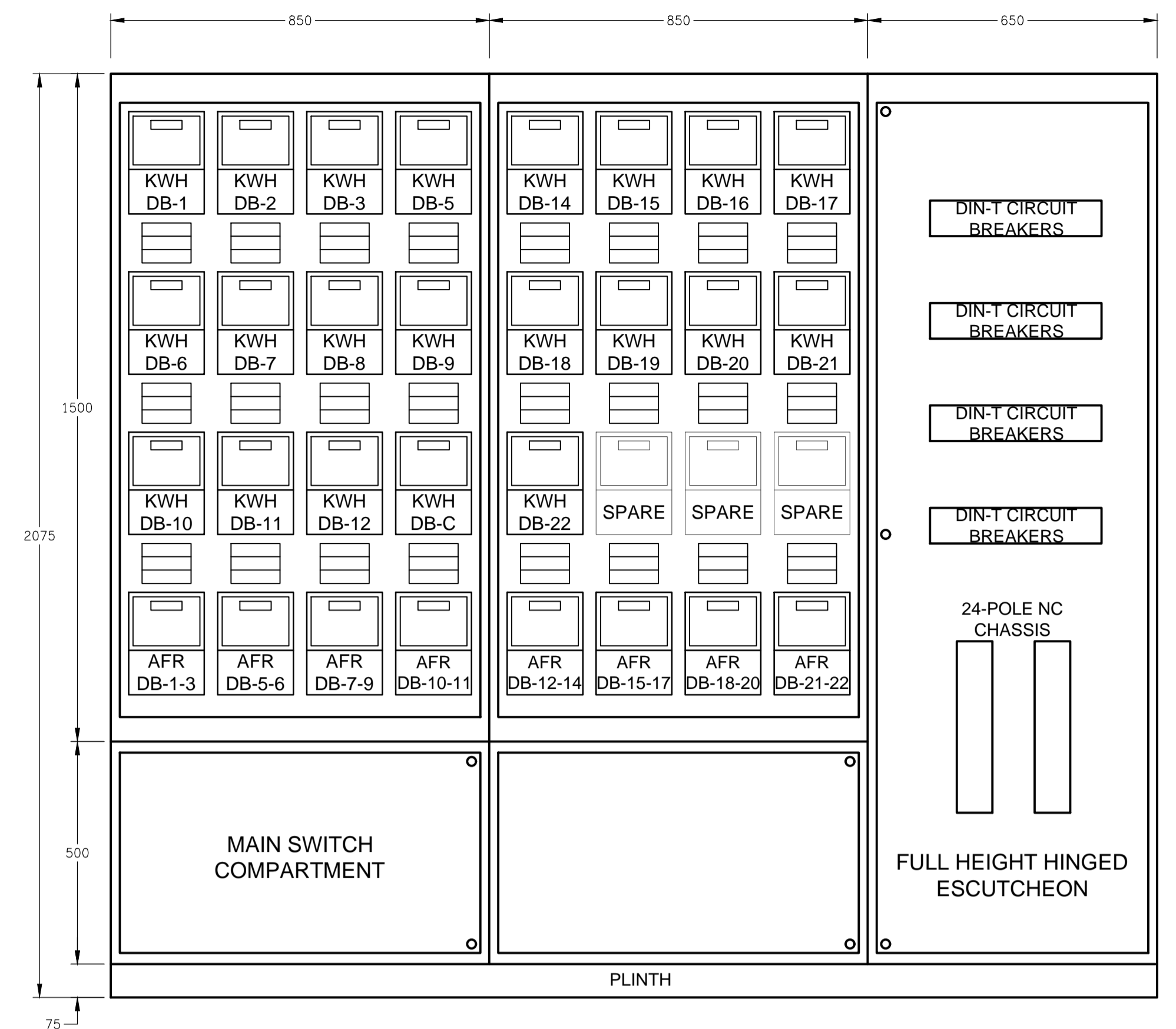
DETAIL B MSB FRONT ELEVATION VIEW NOT TO SCALE
