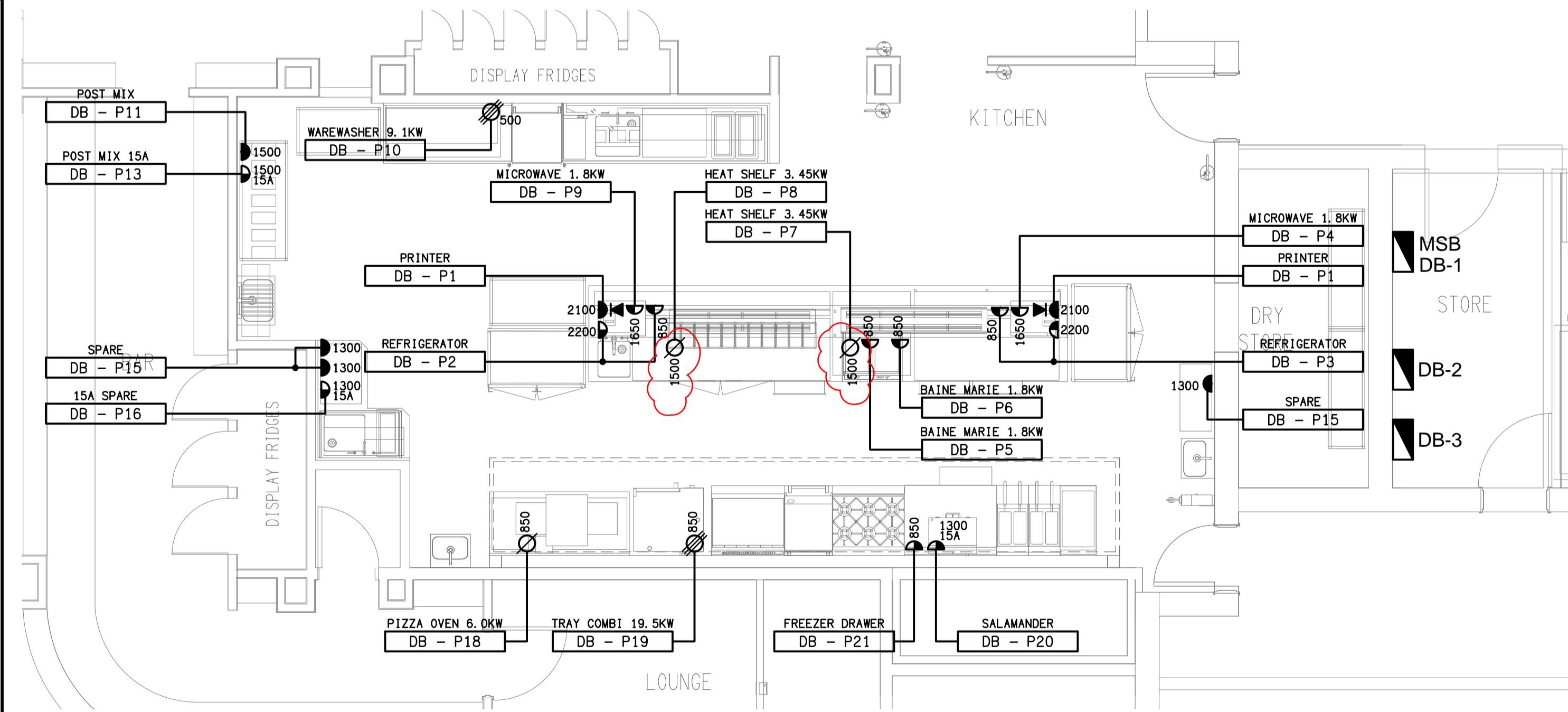
FLOOR PLAN KITCHEN REFURBISHMENT SCALE 1:50
