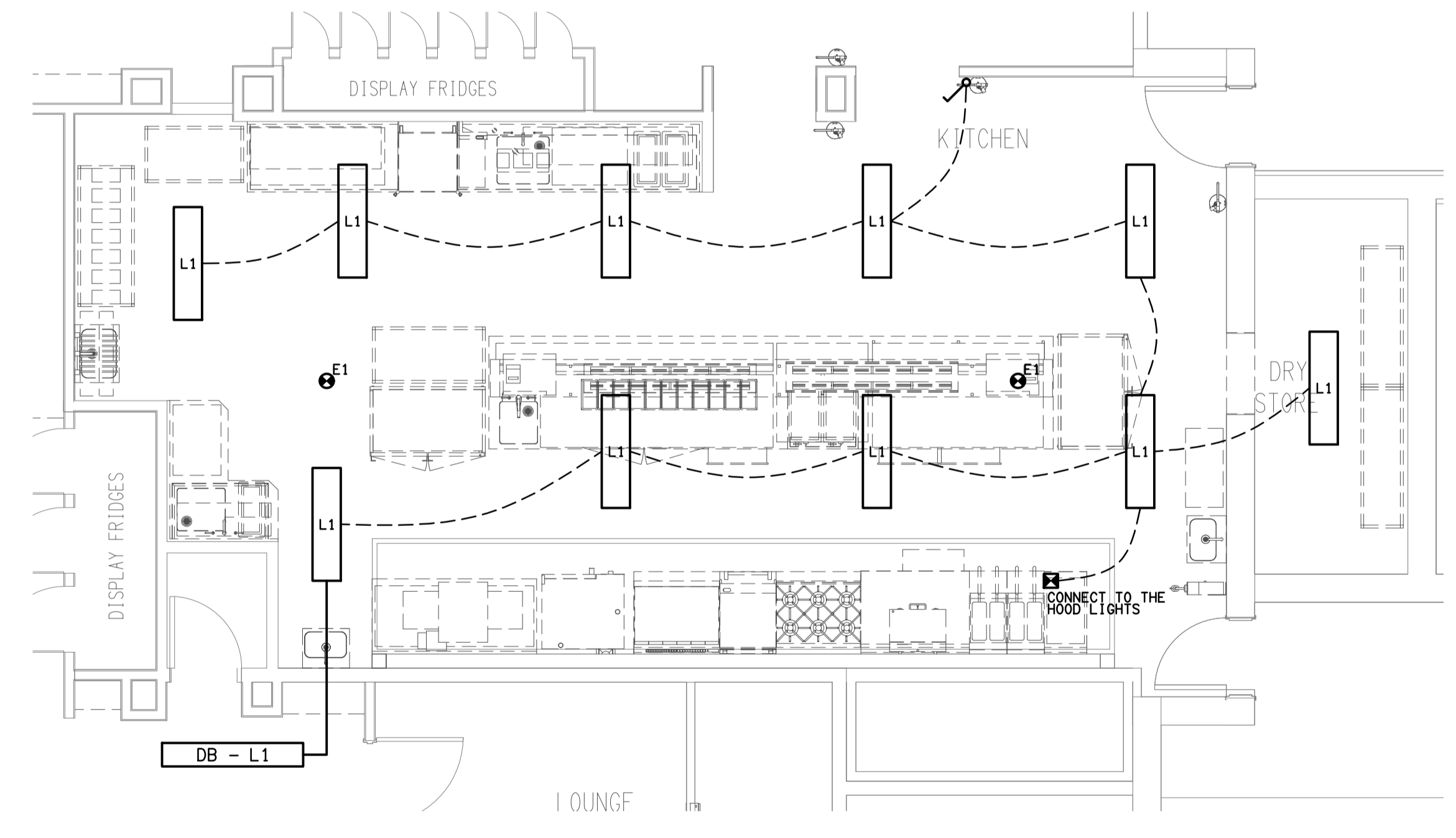
REFLECTED CEILING PLAN KITCHEN REFURBISHMENT SCALE 1:50
