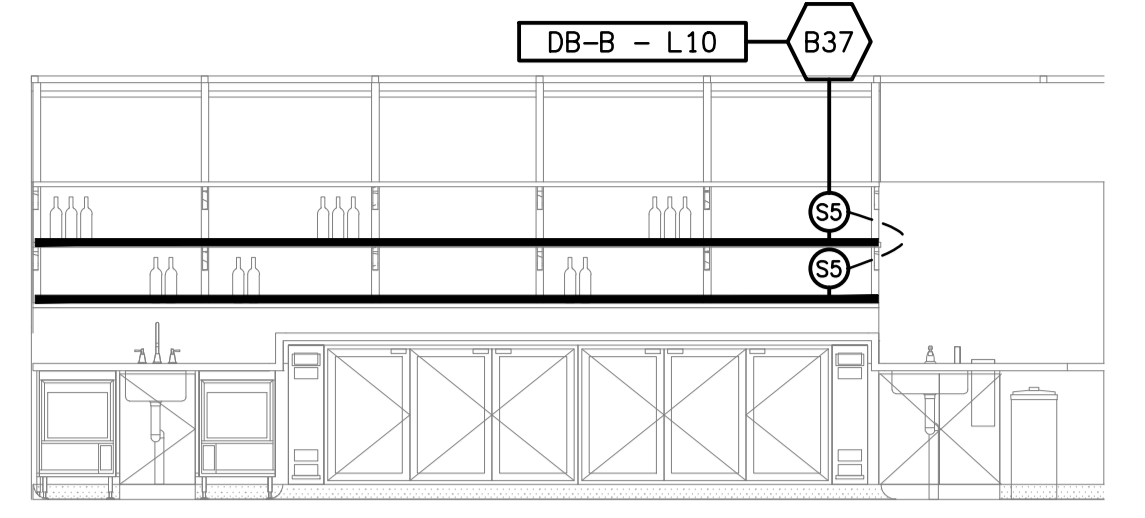
DETAIL A PUBLIC BAR REAR SHELVING ELEVATION SCALE 1:50
