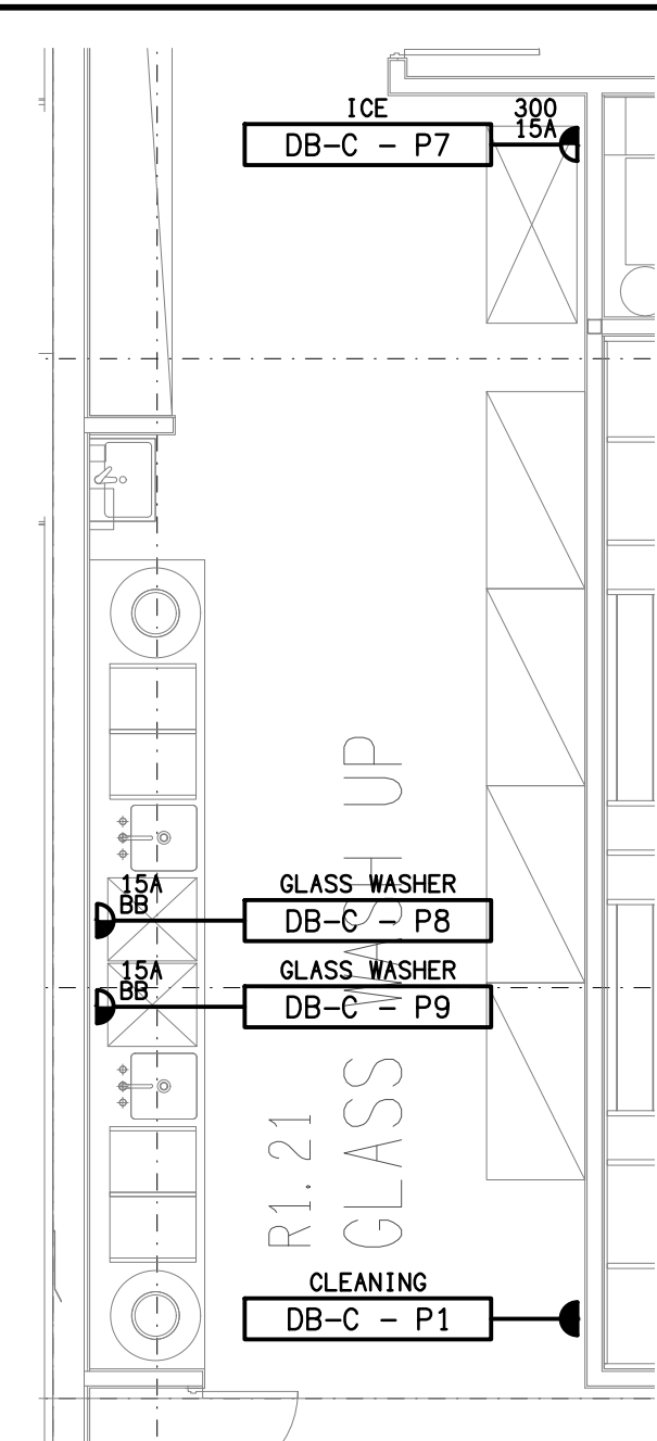
DETAIL A GLASS WASH UP LAYOUT SCALE 1:50
