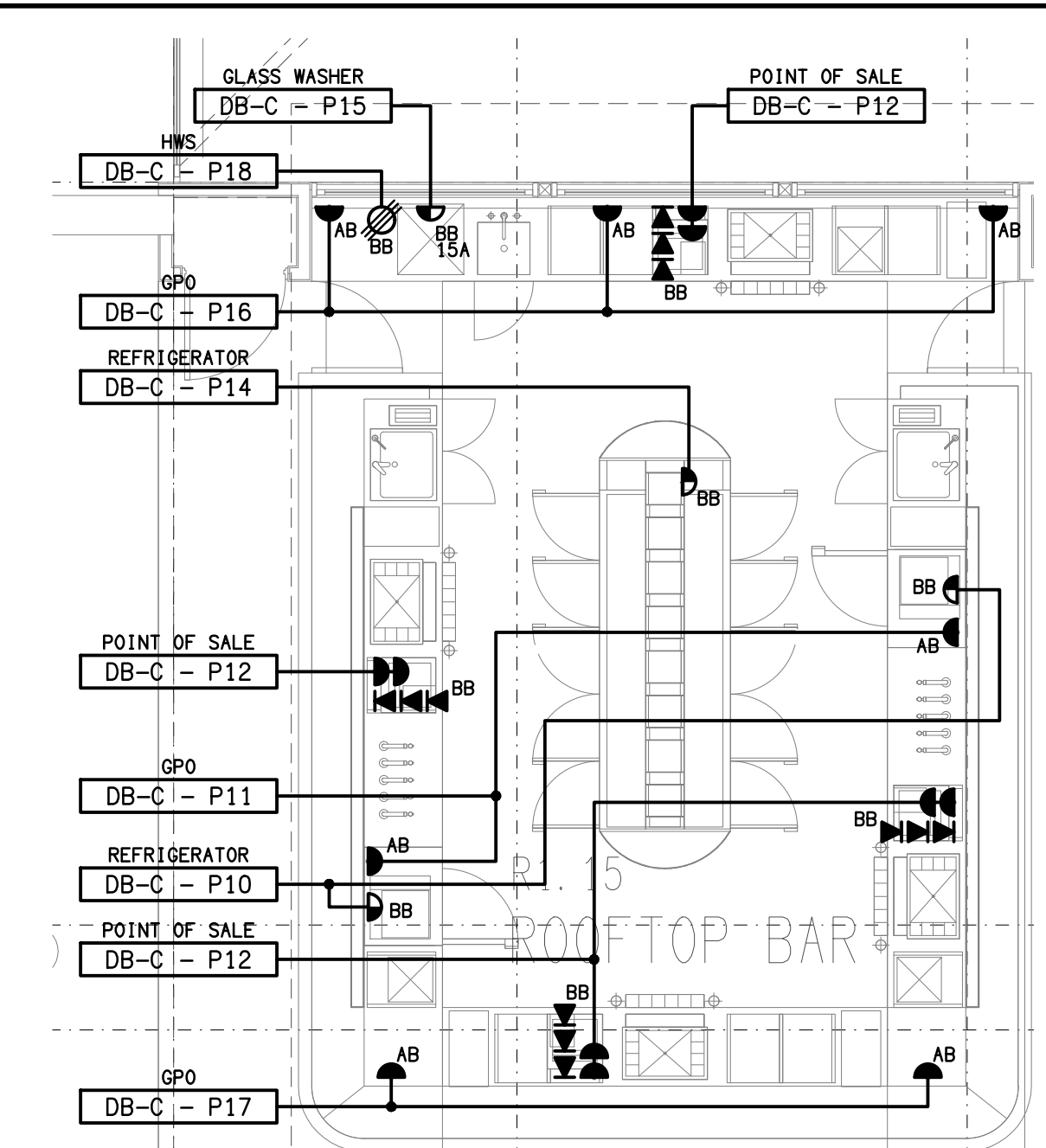
DETAIL B ROOF TOP BAR LAYOUT SCALE 1:50
