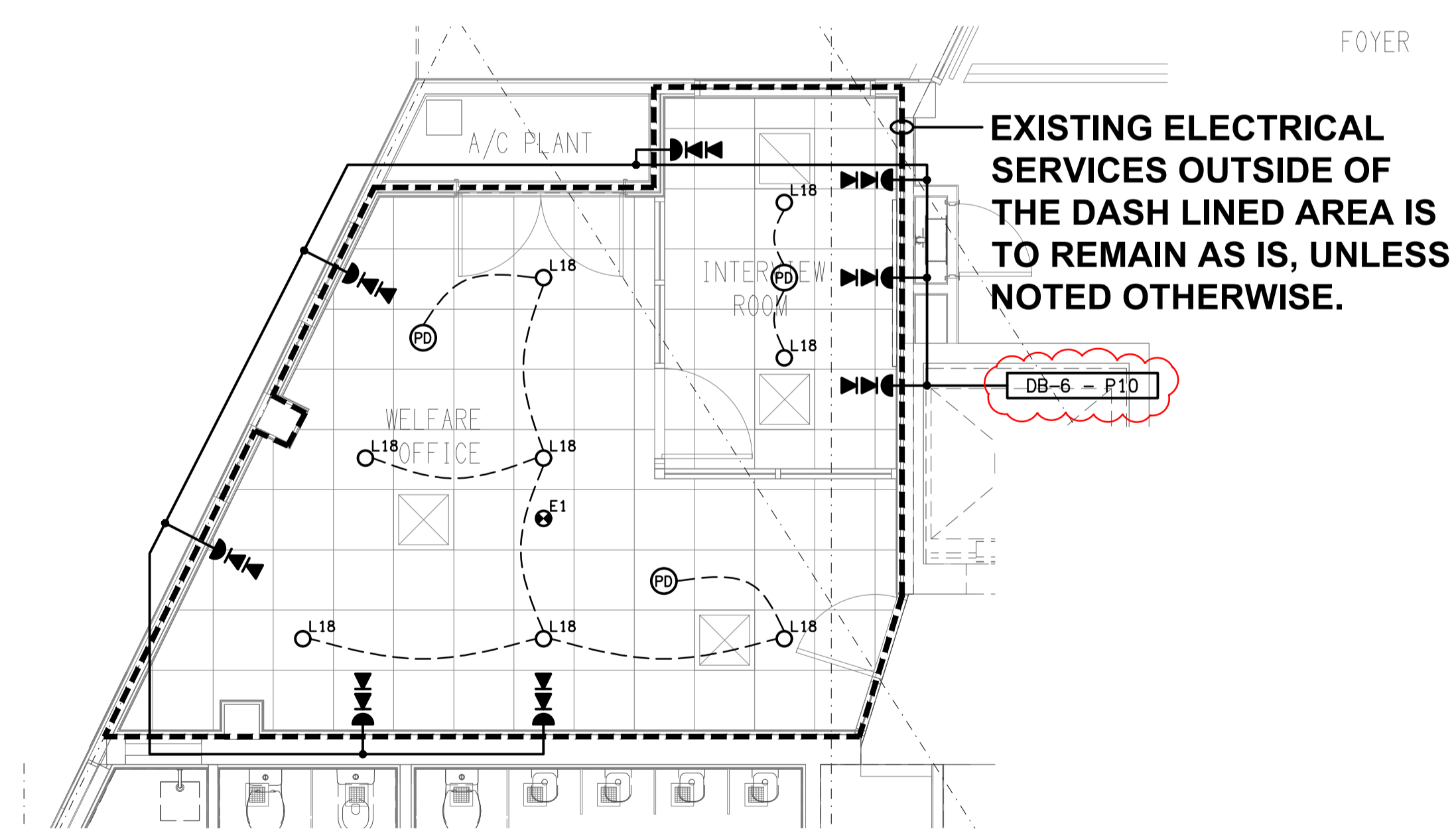
DETAIL A WELFARE OFFICE CEILING PLAN SCALE 1:50
