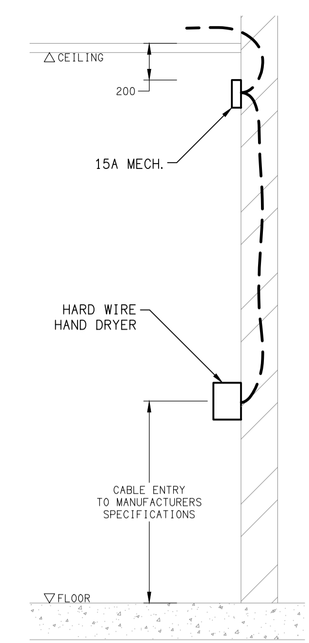
DETAIL HAND DRYER CONNECTION NOT TO SCALE
