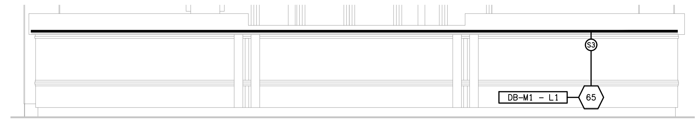
DETAIL 4 SPORTS BAR COUNTER ELEVATION SCALE 1:25
