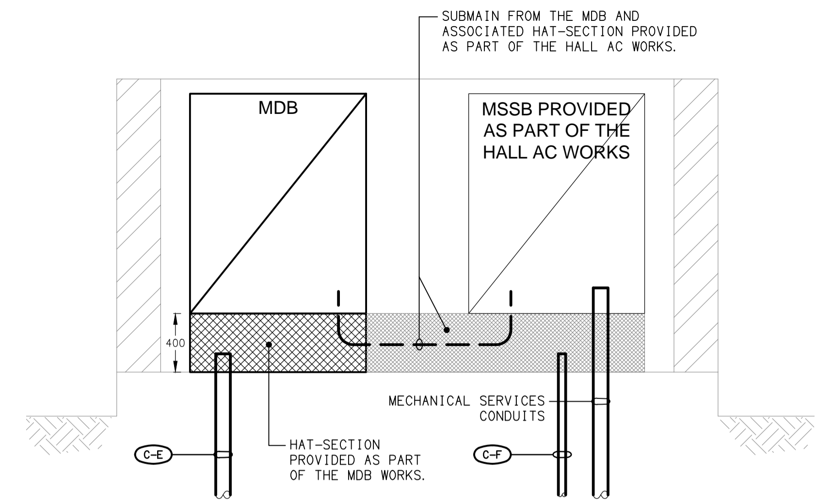
DETAIL A MDB ELEVATION NOT TO SCALE
