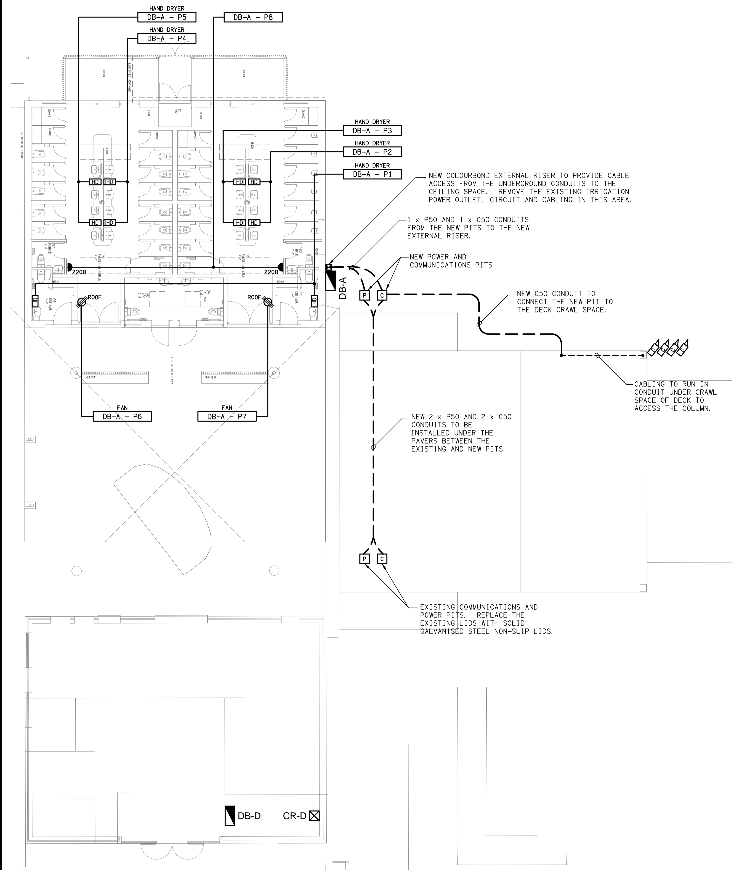
FLOOR PLAN AMENITIES BLOCK UPGRADE SCALE 1: 100
