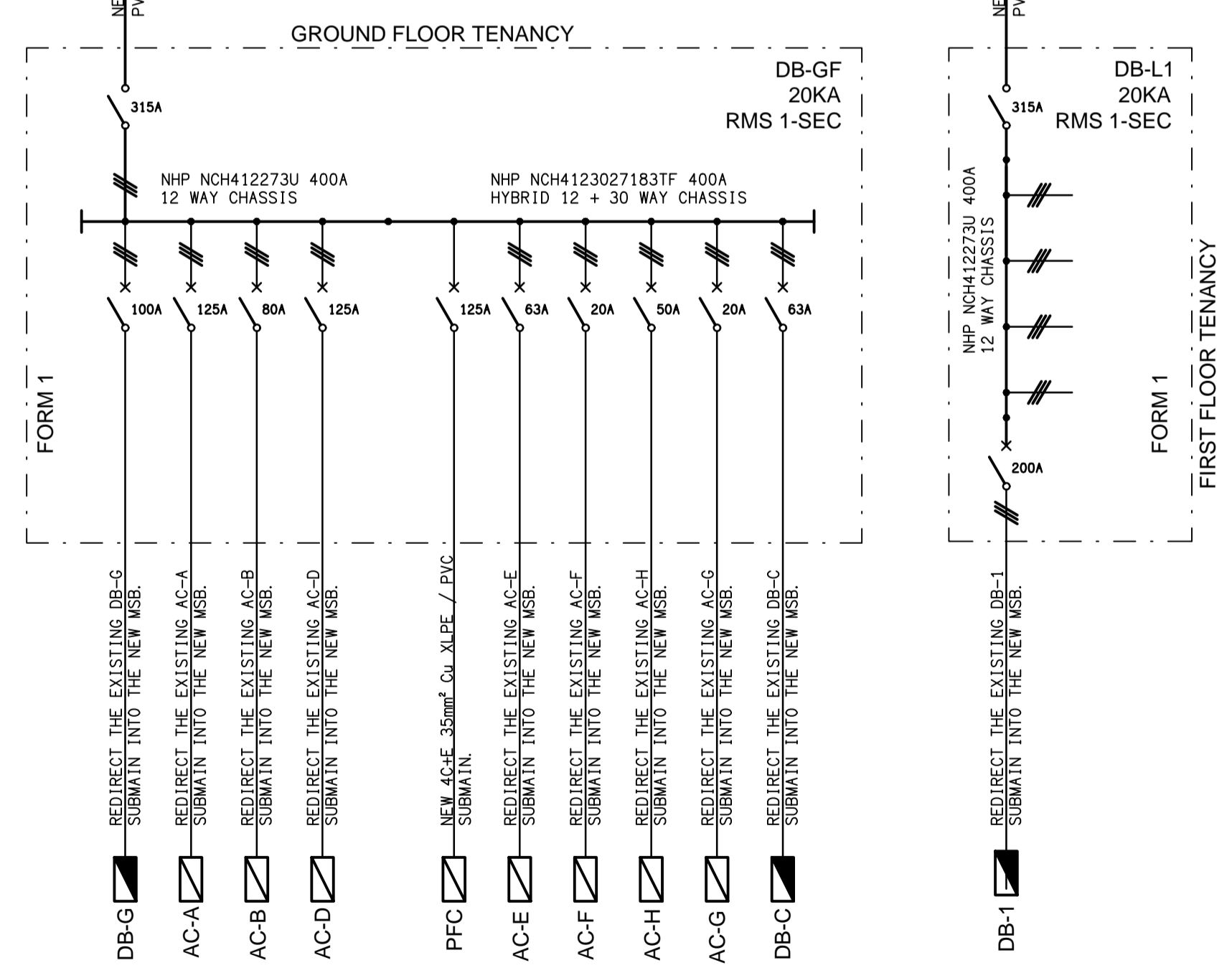
PROPOSED SCHEMATIC POWER CONFIGURATION NOT TO SCALE
